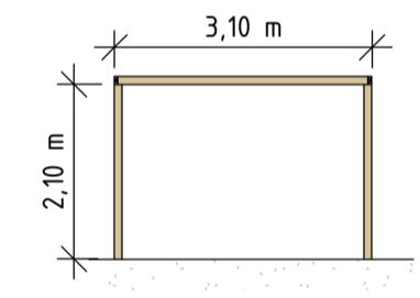
PERGOLA GAVEL 1
