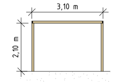
PERGOLA GAVEL 2
